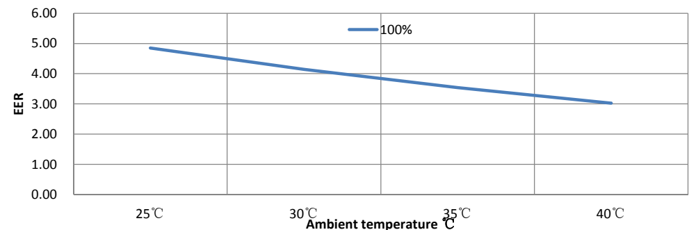
IXCR80 EER Curve
