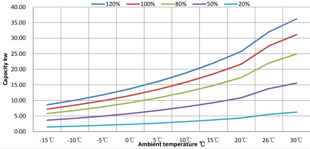
IXCR80 COP Curve
