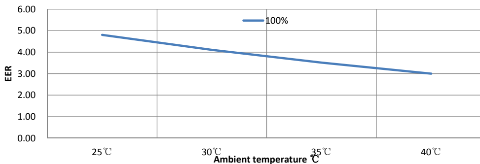
IXCR26 EER Curve
