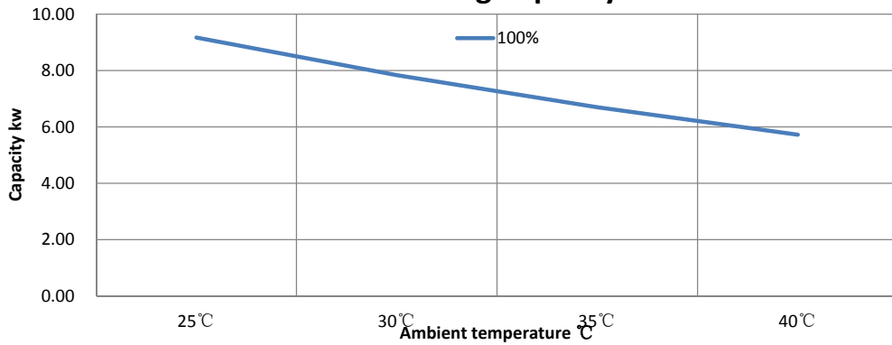
IXCR46 Cooling Capacity Curve
