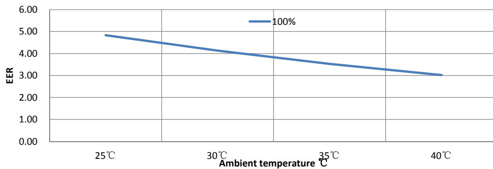
IXCR66 EER Curve
