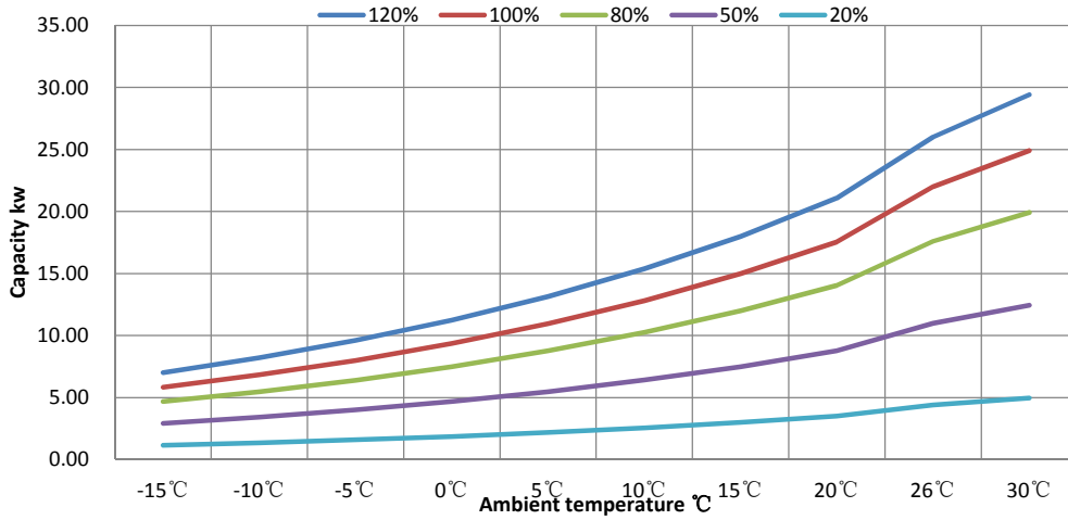
IXCR66 COP Curve
