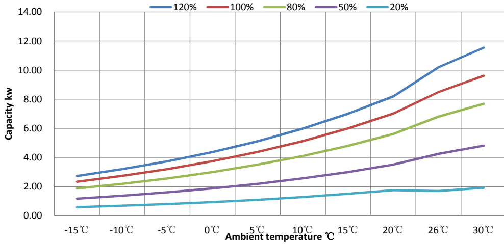
IXCR26 COP Curve
