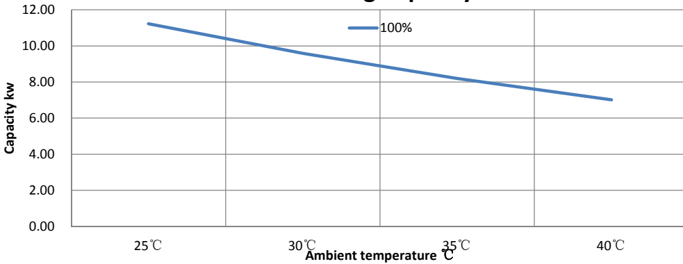
IXCR56 Cooling Capacity Curve
