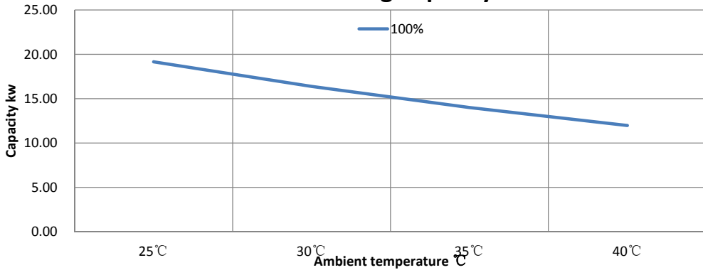
IXCR80T Cooling Capacity Curve
