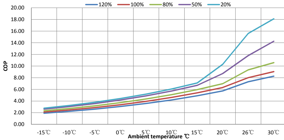
IXCR26 Cooling Capacity Curve
