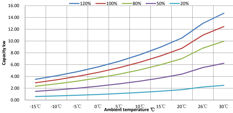
IXCR36 COP Curve
