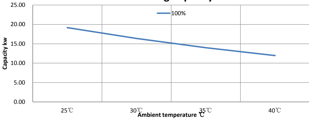
IXCR80 Cooling Capacity Curve
