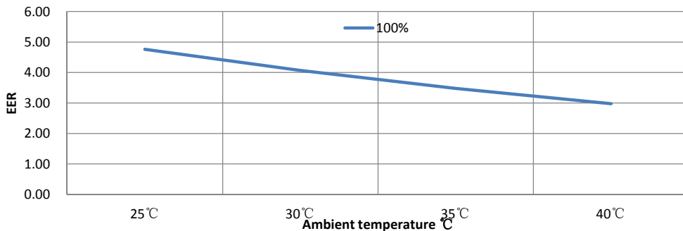
IXCR56 EER Curve
