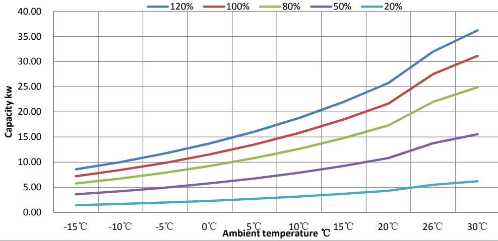
IXCR80T COP Curve
