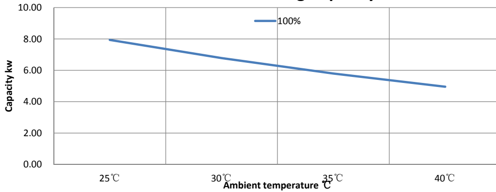
IXCR36 Cooling Capacity Curve
