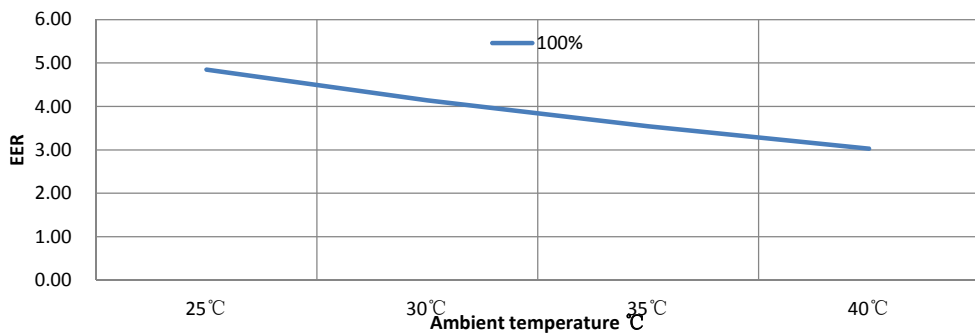
IXCR80T EER Curve
